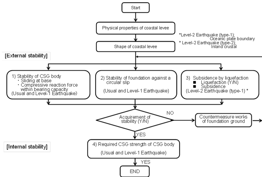
Fig.3 Structure analysis flow Flux d'analyse de structure
