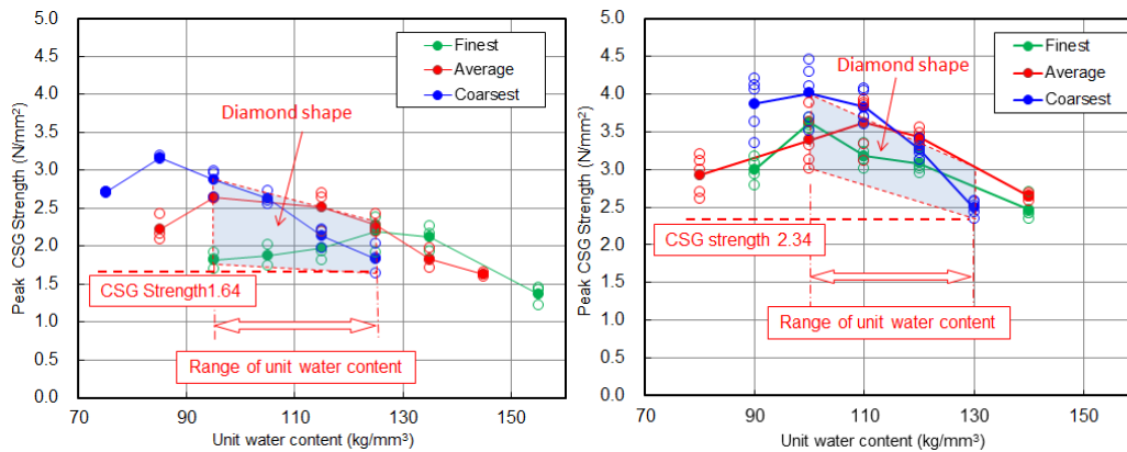
(1) Unit cement content of 40 kg/m 3 (2) Unit cement content of 60kg/m 3 Fig. 9
