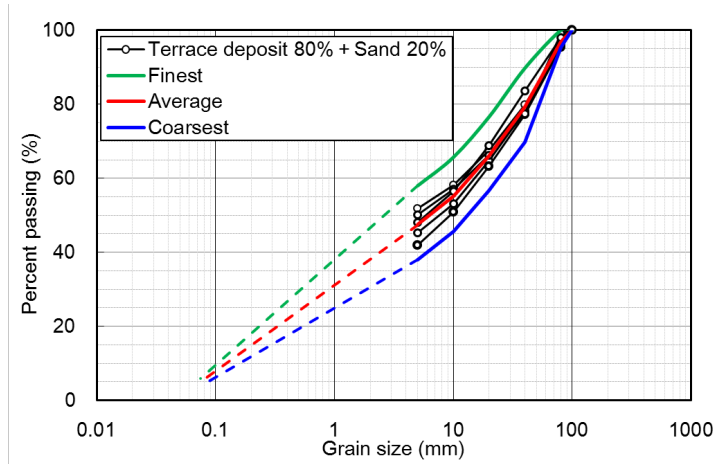
(1) Terrace deposit 80% + In-situ sand 20%
